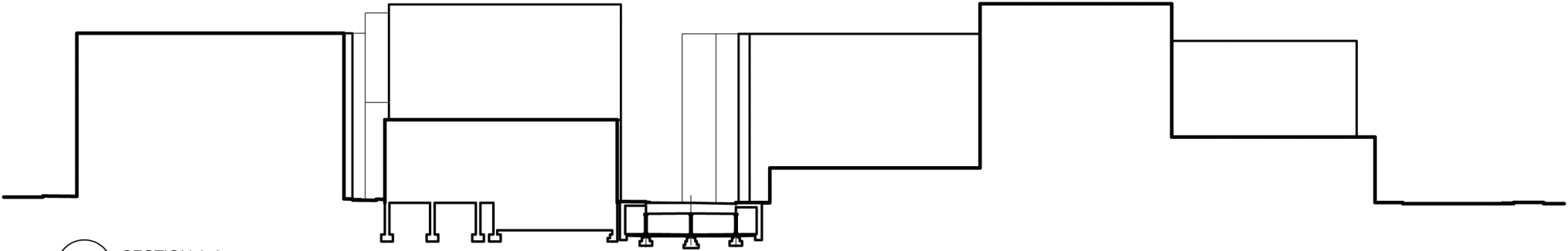
1 SECTION A-A \frac{1}{64}'' = 1'-0''
